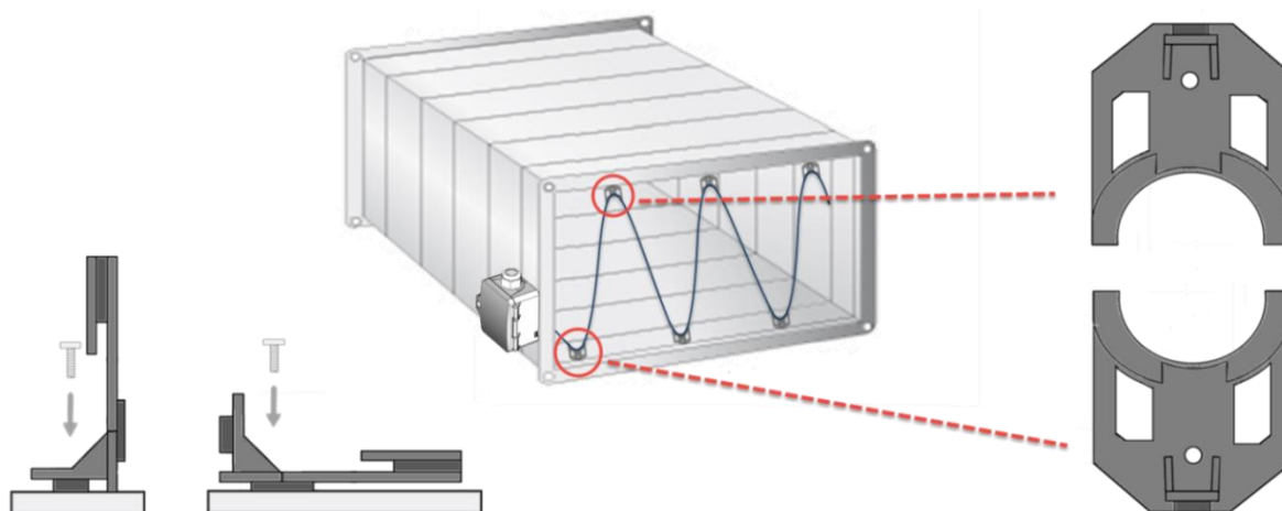
Vertical mounting Horizontal mounting
