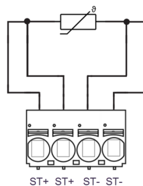
fig. (terminal assignment passive sensor)
