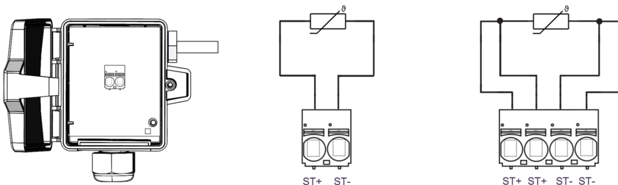
fig. (terminal assignment passive sensor)
