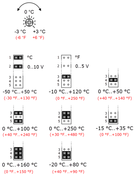
fig. (Measuring range and offset adjustment, default settings: -50 °C..+50 °C | 0 K)
