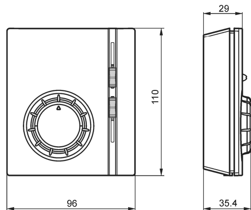
Room thermostat
